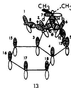
Figure 4. Basis sets for SCF-CI calculations for species 3, 17, and 13.
