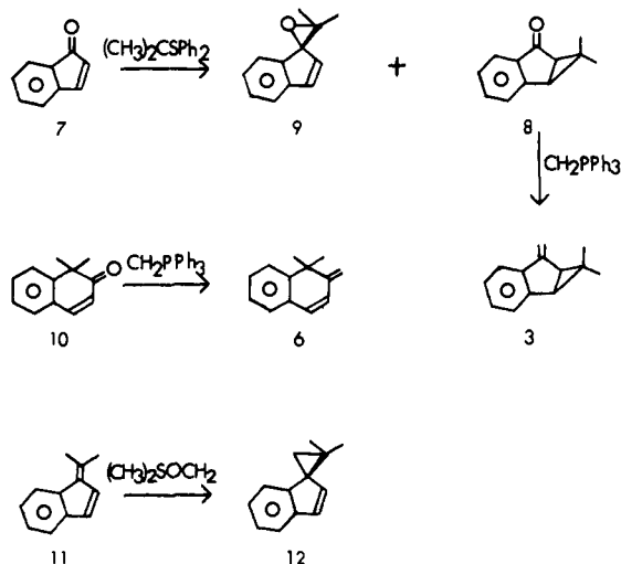
Scheme I. New Syntheses of Photochemical Reactants and Products
