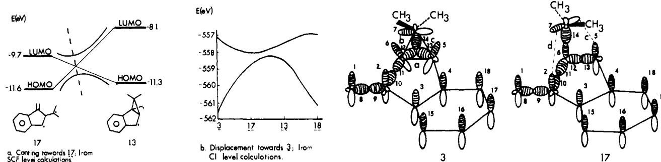
Figure 3. Energetics, canting, and displacement of the bifunnel.
